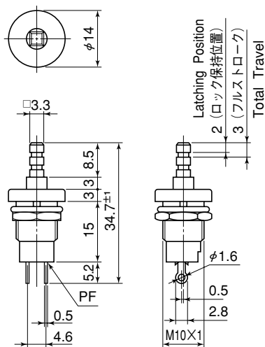
Solder Terminal
