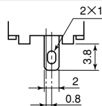
Solder Terminal
